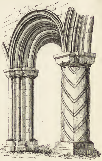
42. Lindisfarne Priory, Durham, A.D. 1094—1120. Arch richly moulded, one pier with shafts attached, the other with zig-zag fluting.
